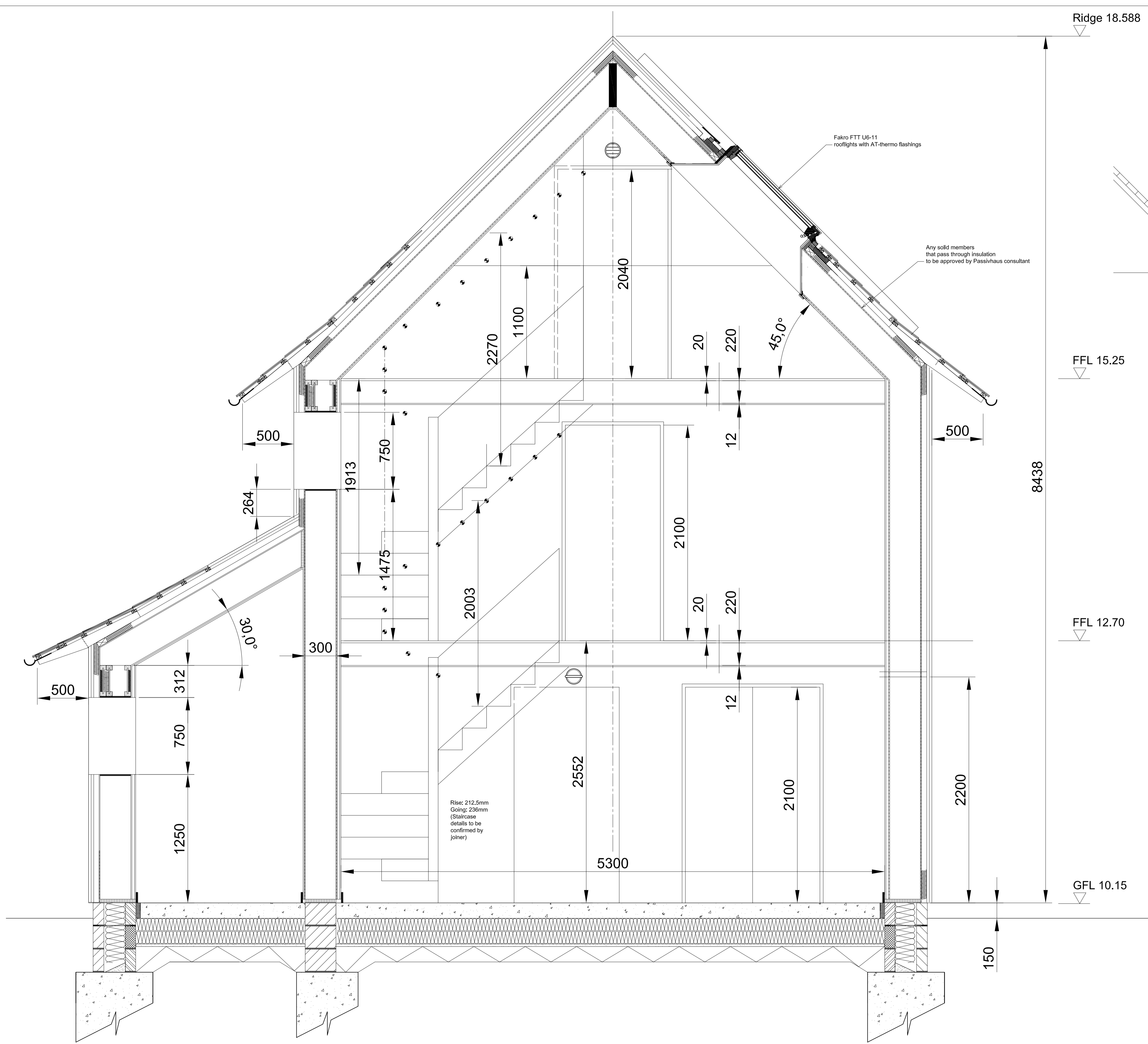
SECTION (SCALE 1:20)
